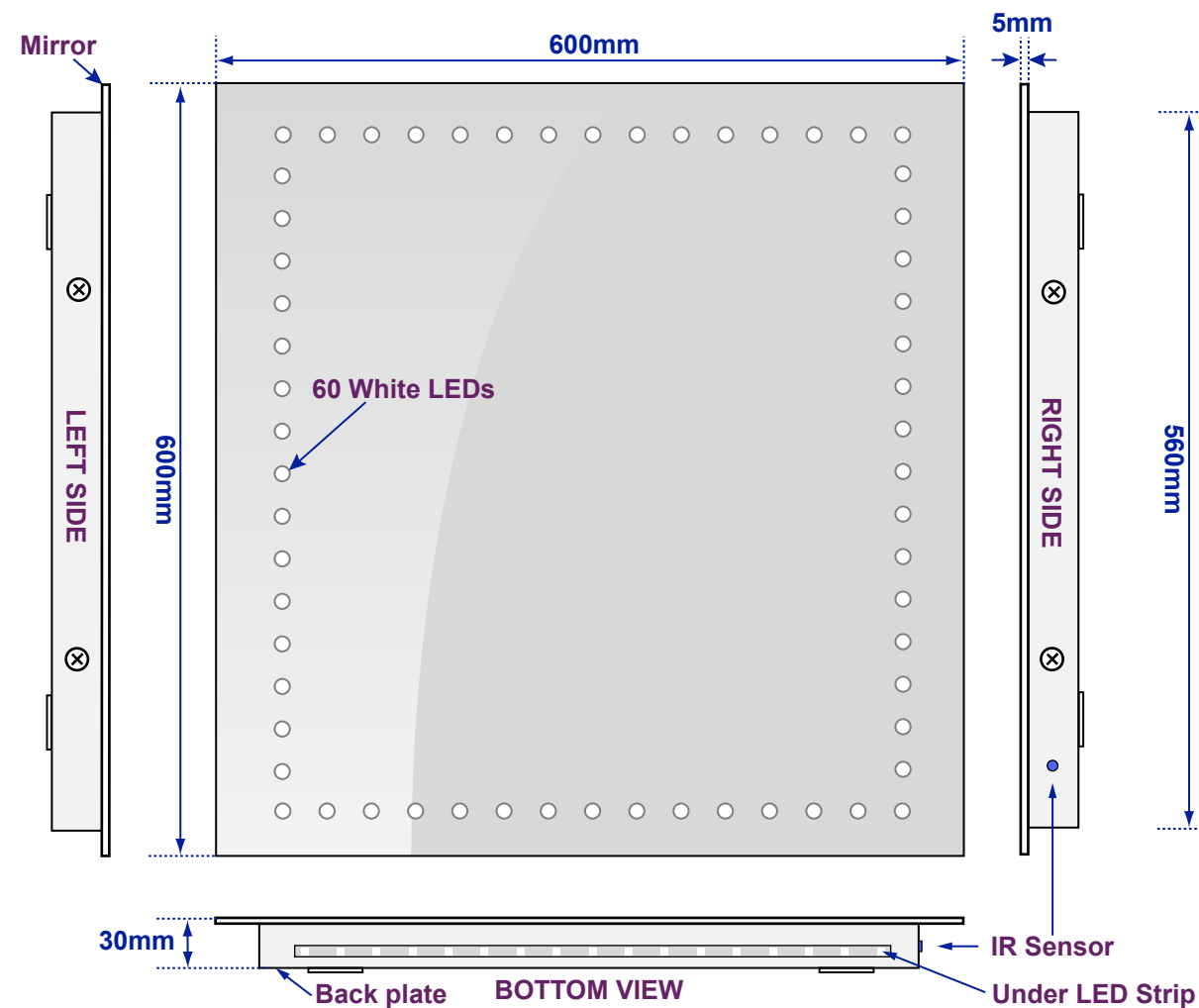
Views of complete assembly - With Mirror
