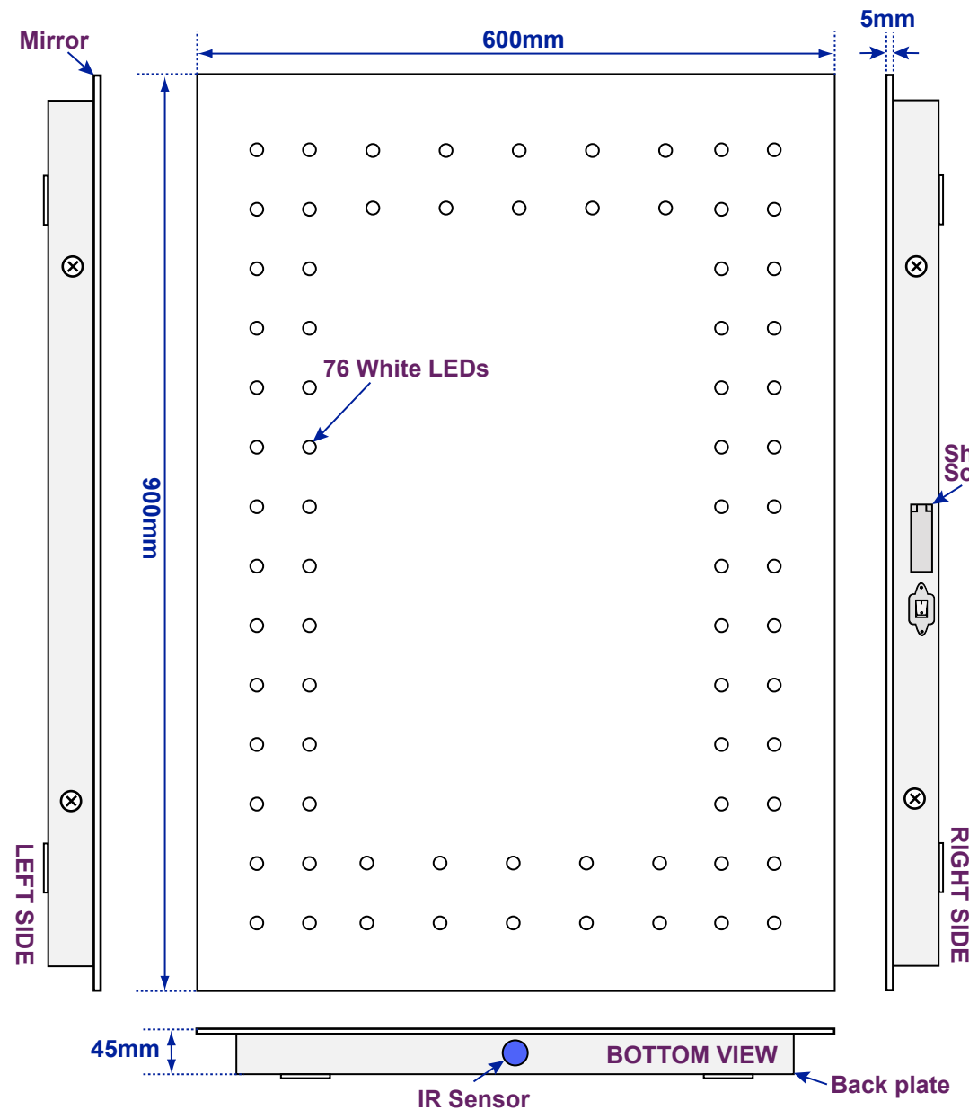
Views of complete assembly - With Mirror
