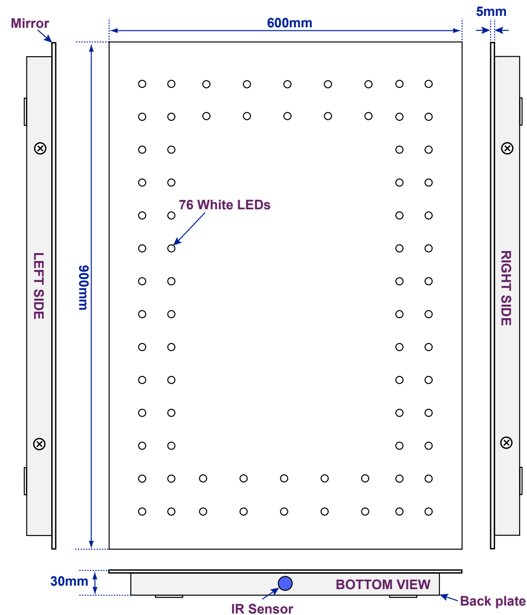
Views of complete assembly - With Mirror
