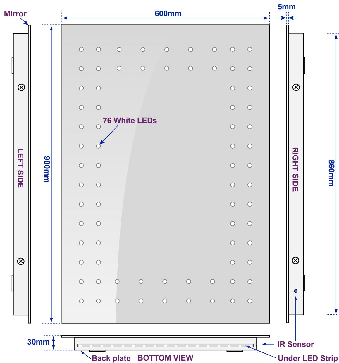
Views of complete assembly - With Mirror
