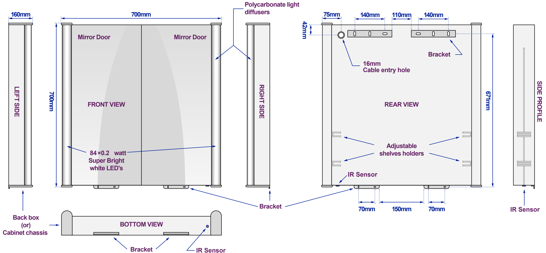
Views of complete assembly - With Mirror Door(s)
