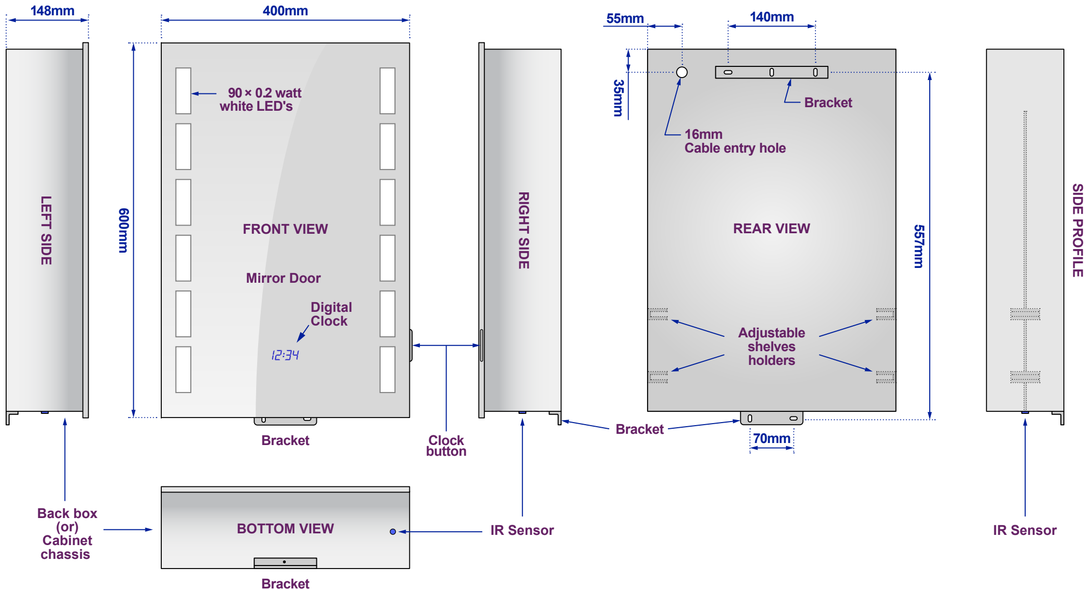
Views of complete assembly - With Mirror Door(s)/Panel(s)
