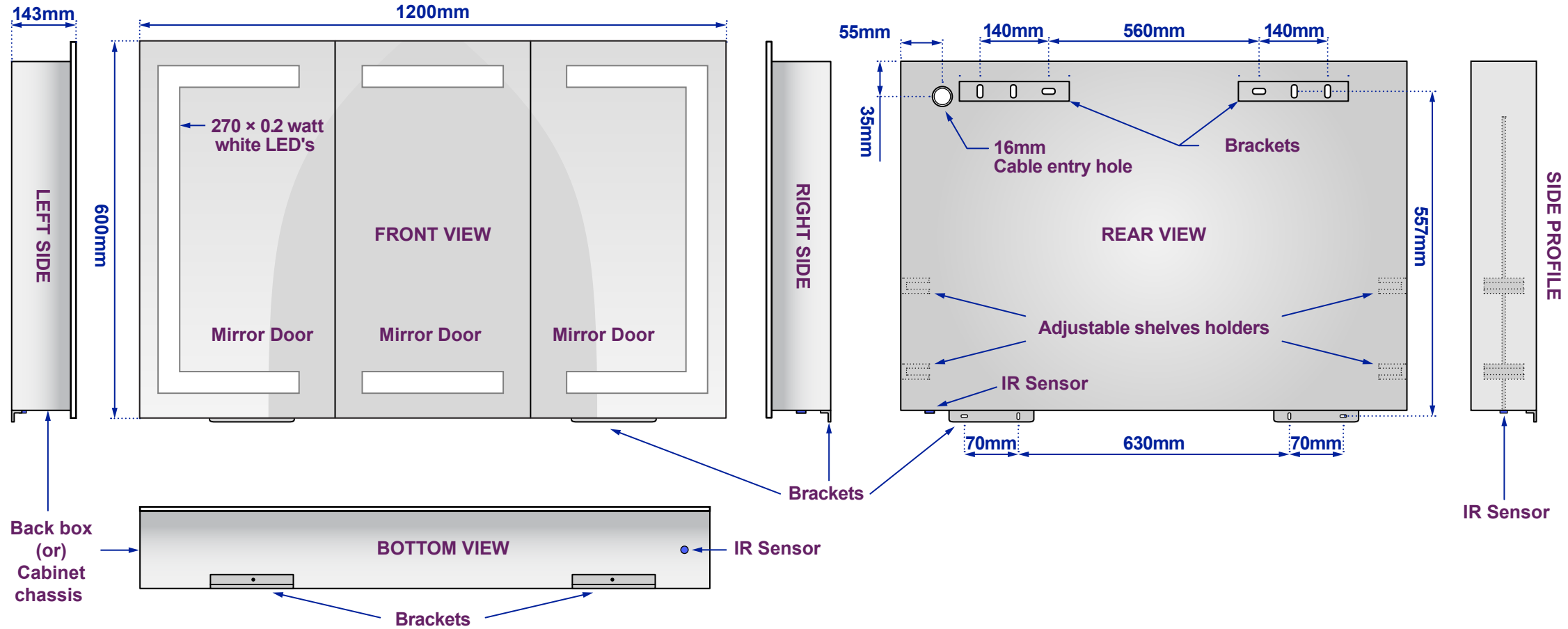
Views of complete assembly - With Mirror Door(s)/Panel(s)
