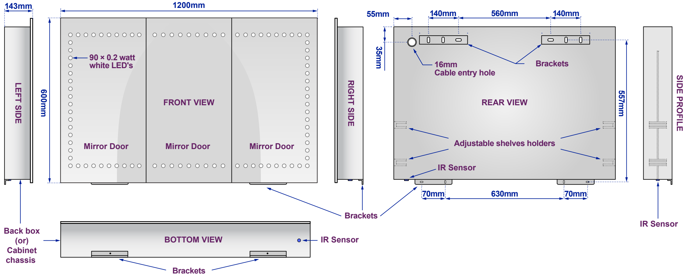
Views of complete assembly - With Mirror Door(s)/Panel(s)
