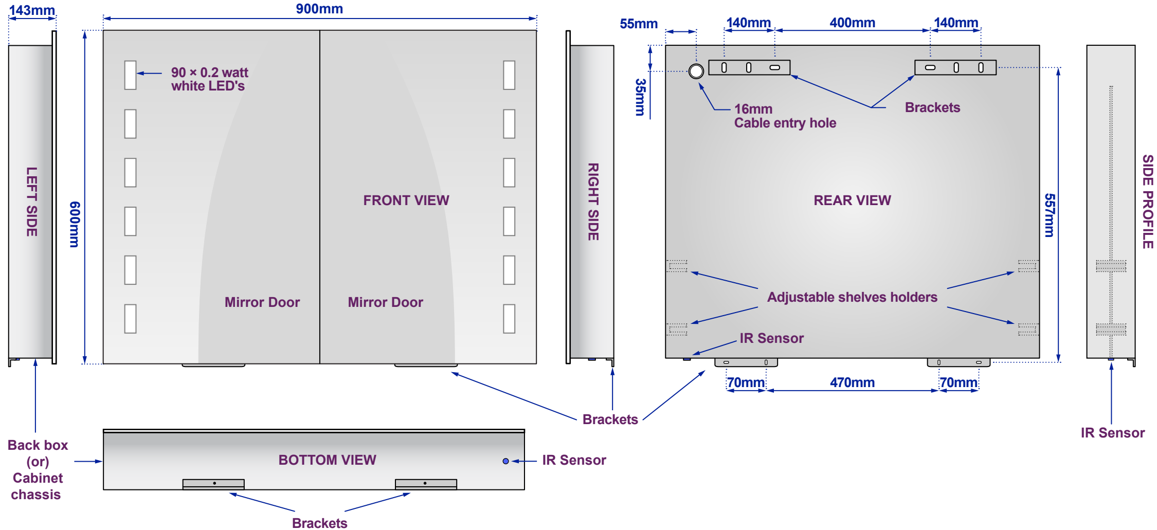
Views of complete assembly - With Mirror Door(s)/Panel(s)
