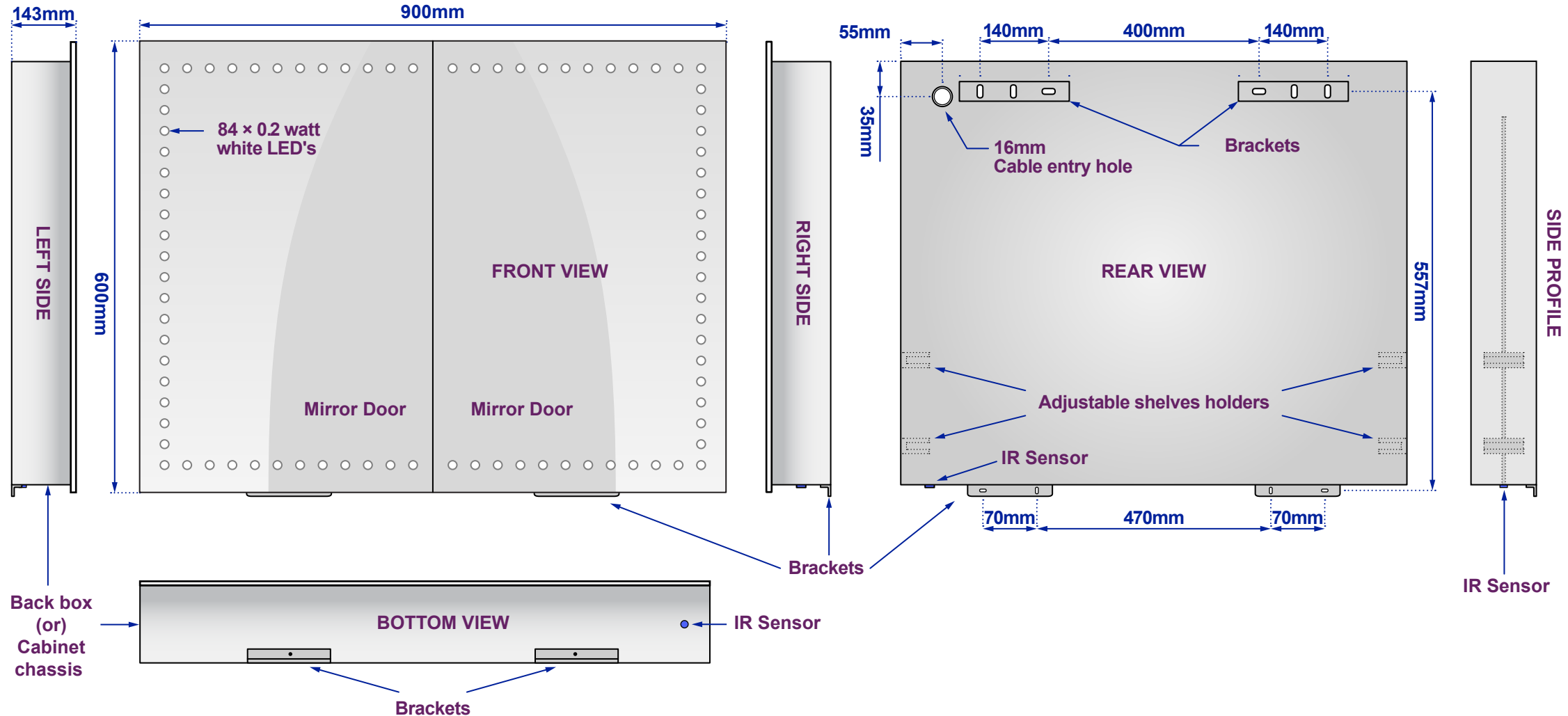
Views of complete assembly - With Mirror Door(s)/Panel(s)
