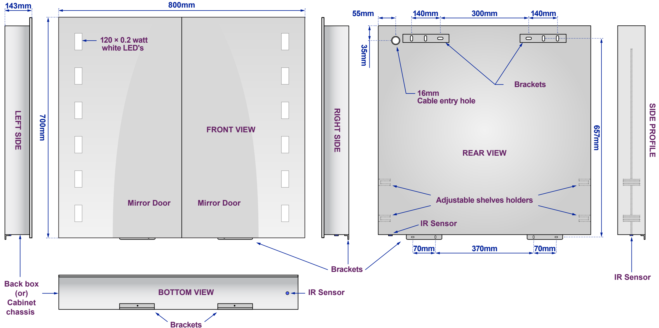
Views of complete assembly - With Mirror Door(s)/Panel(s)
