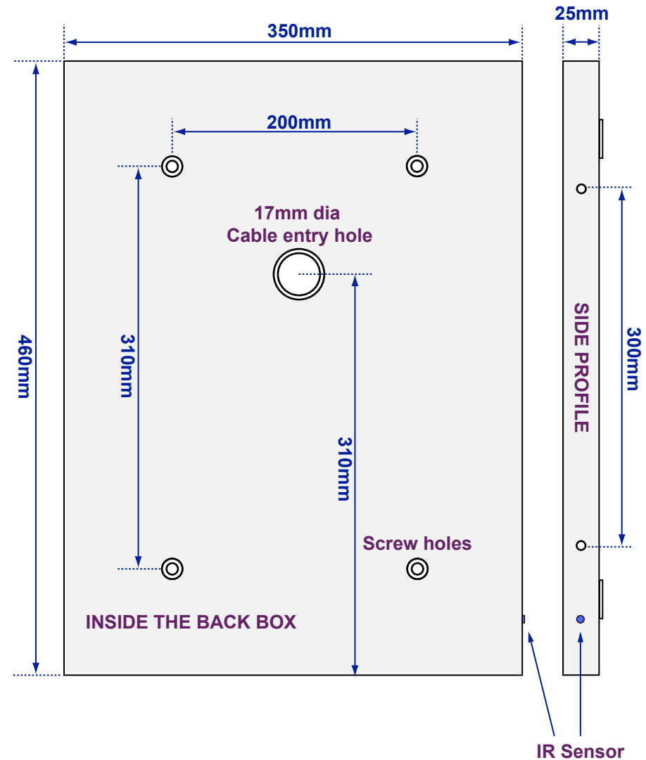
Views of Back plate - Without Mirror
