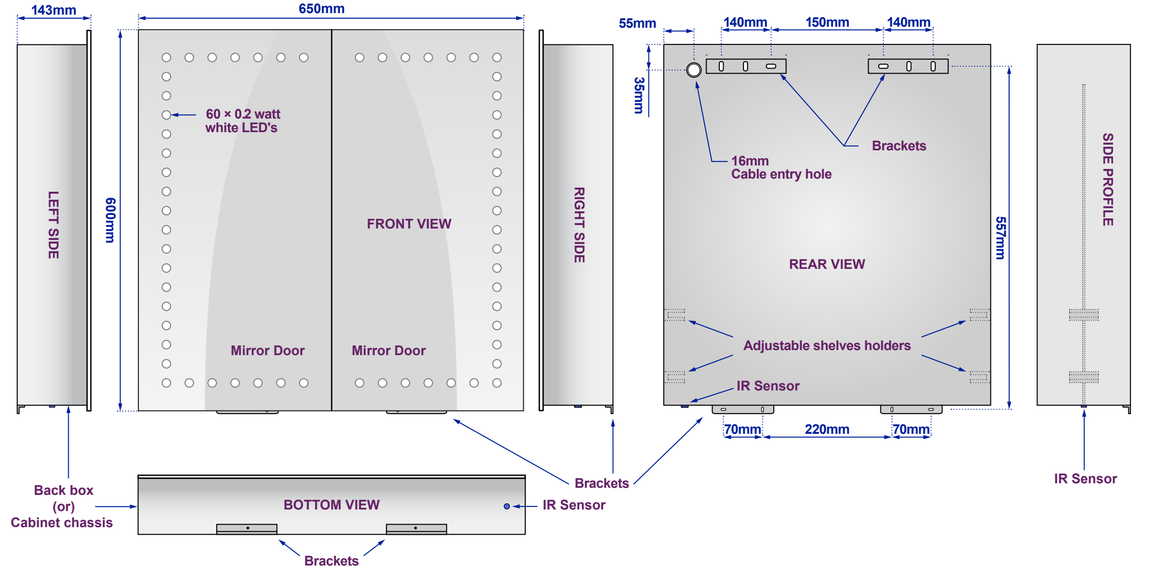
Views of complete assembly - With Mirror Door(s)/Panel(s)
