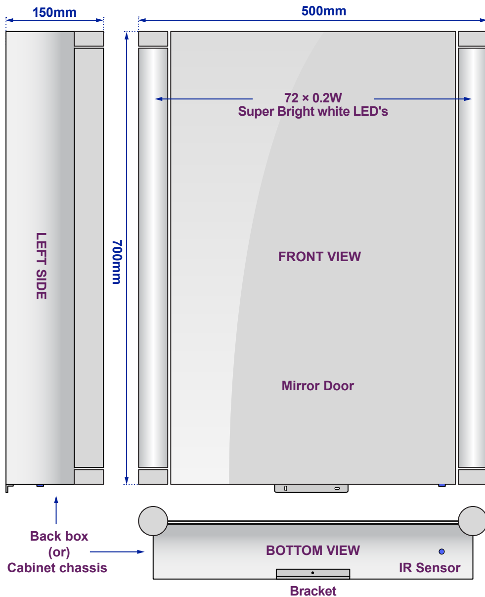
Views of complete assembly - With Mirror Door(s)/Panel(s)
