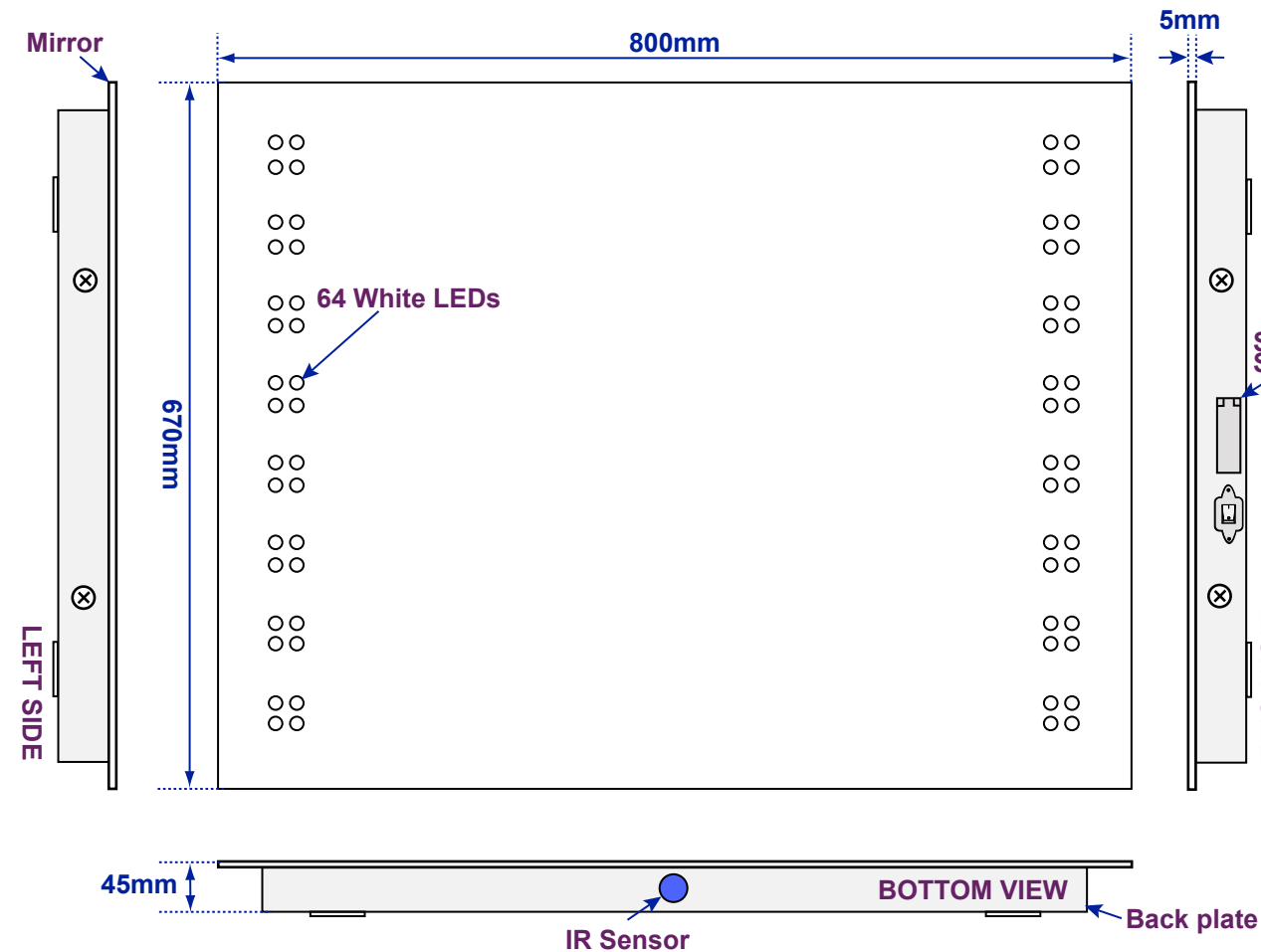
Views of complete assembly - With Mirror
