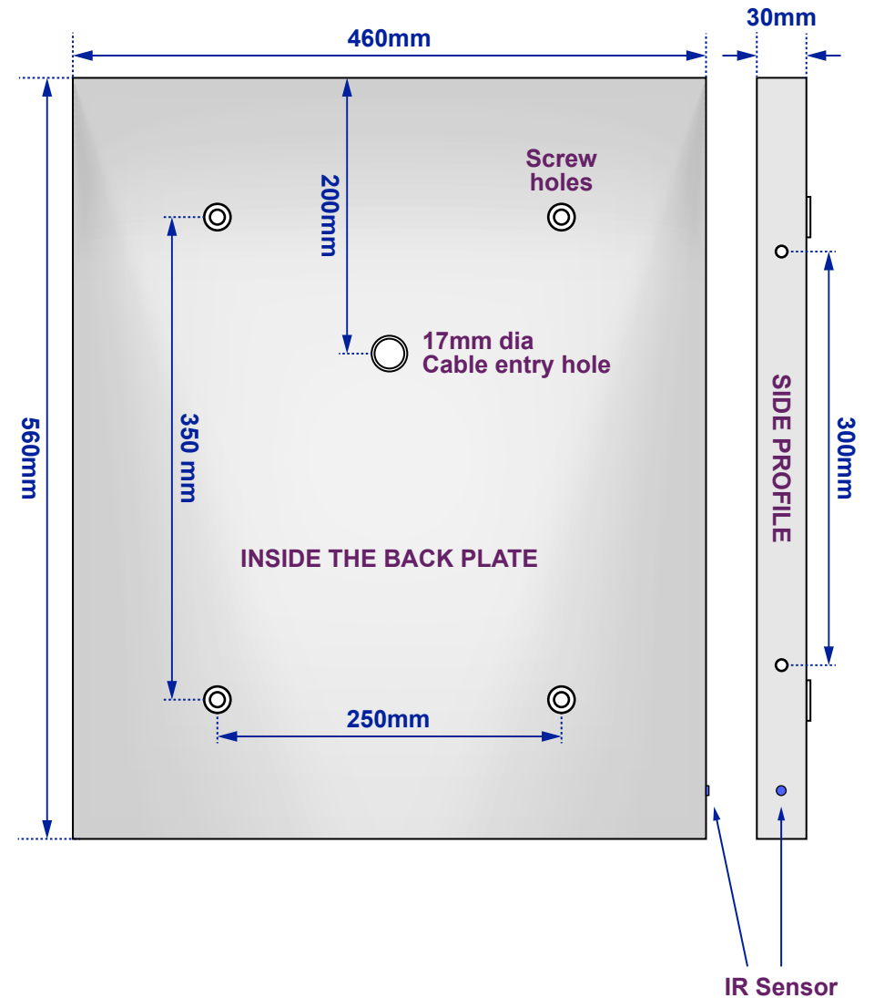
Views of Back plate - Without Mirror
