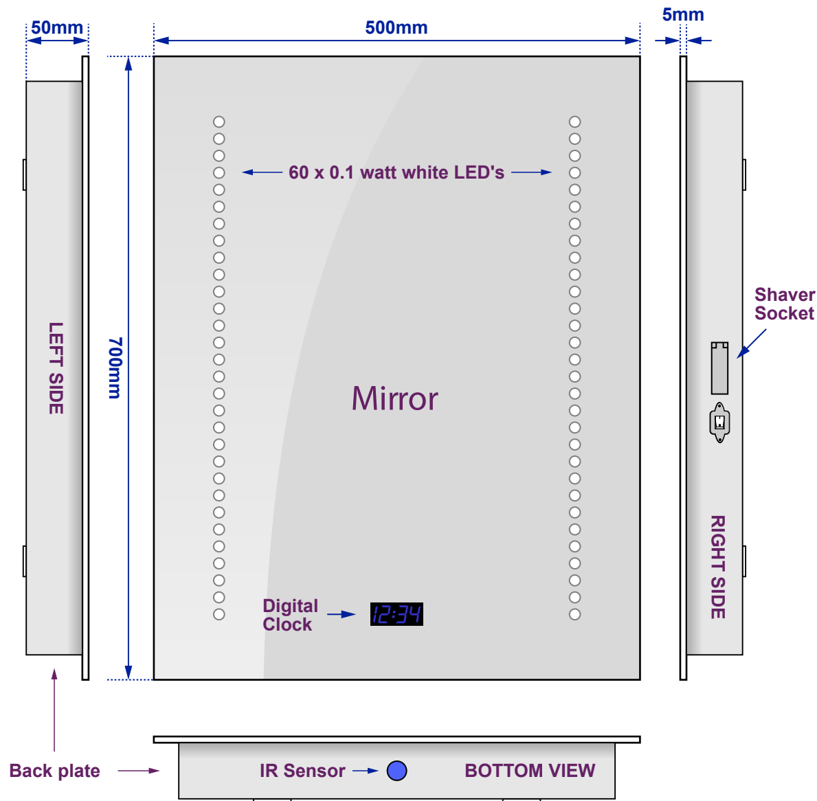
Views of complete assembly - With Mirror
