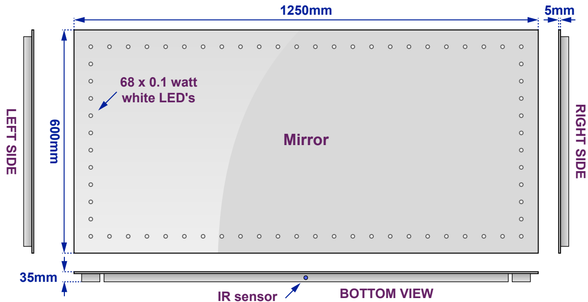
Views of complete assembly
