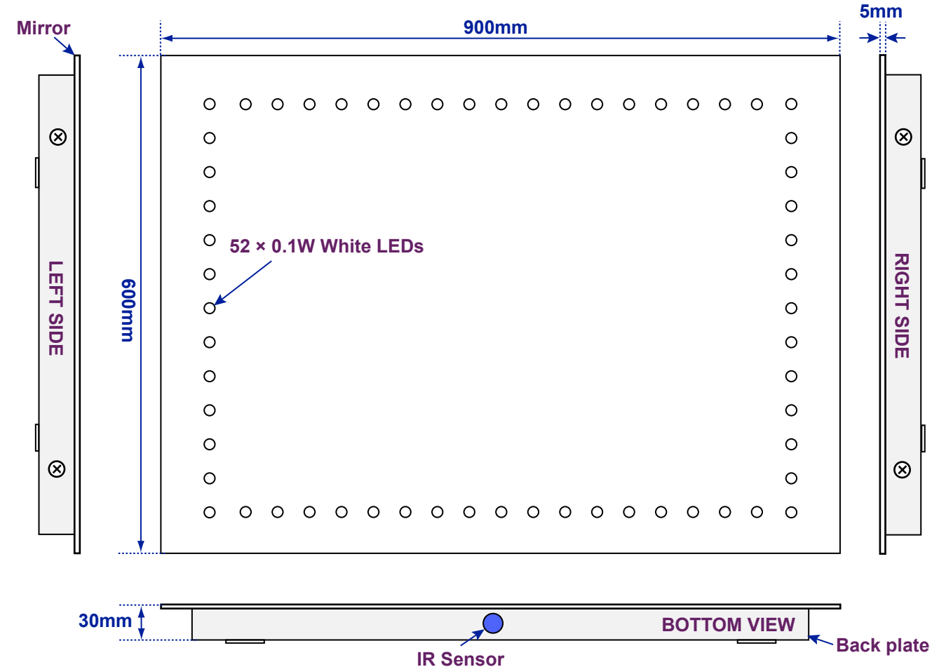
Views of complete assembly - With Mirror
