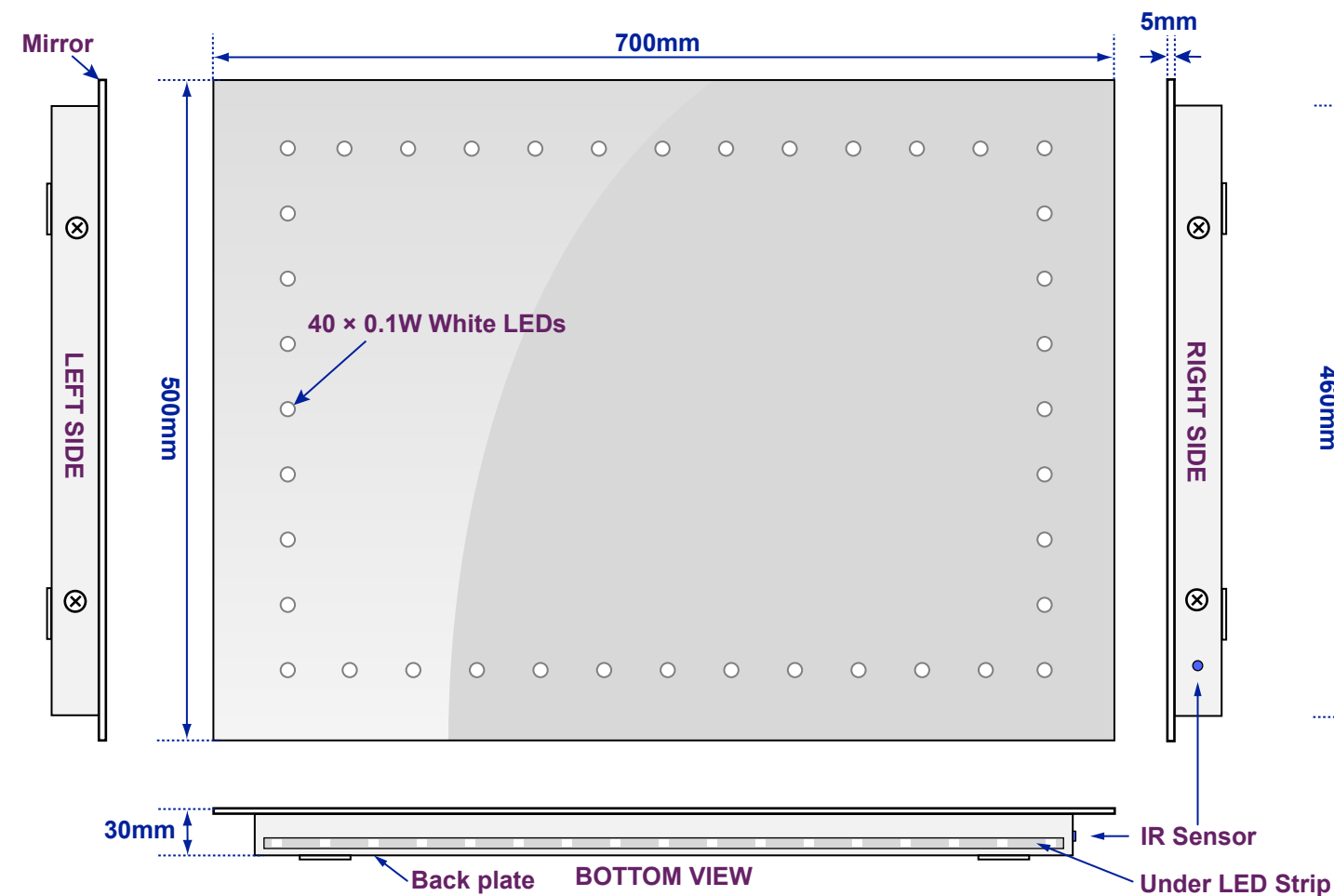
Views of complete assembly - With Mirror
