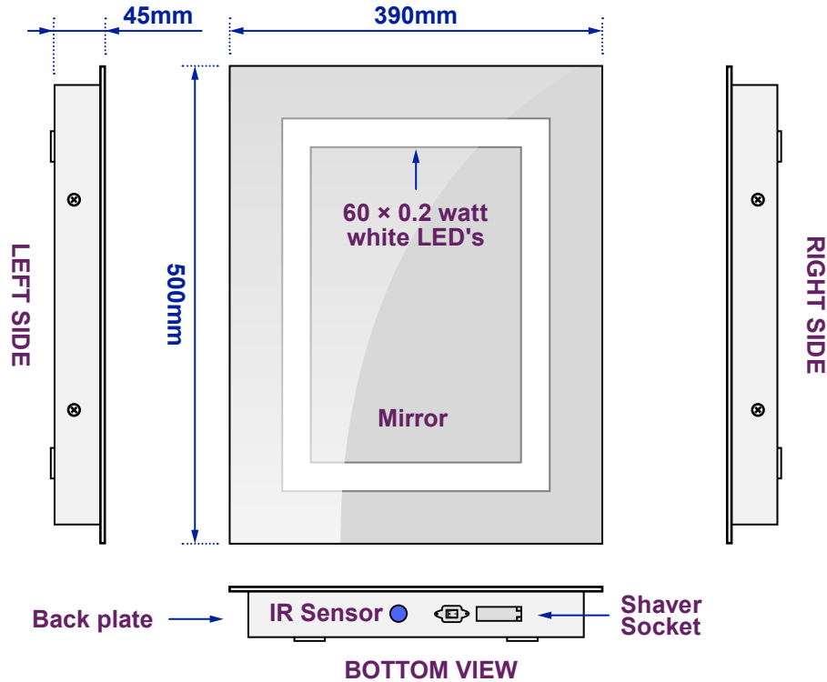
Views of complete assembly - With Mirror
