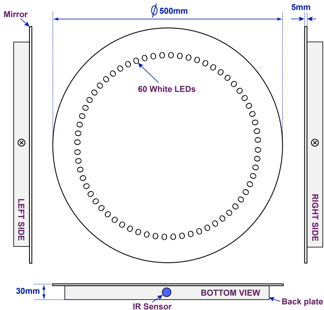
Views of complete assembly - With Mirror
