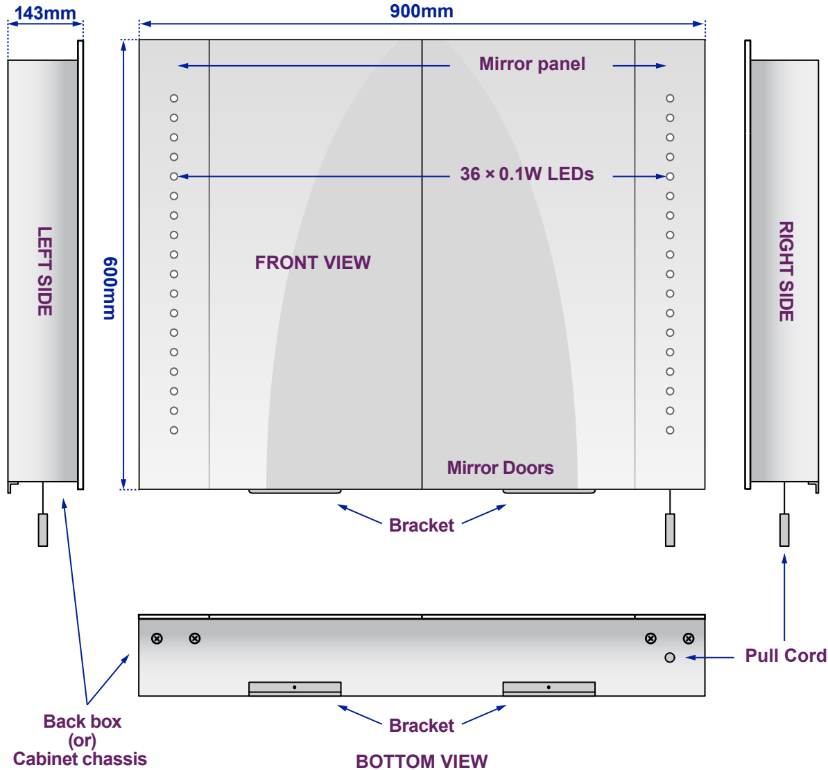
Views of complete assembly - With Mirror Door(s)/Panel(s)
