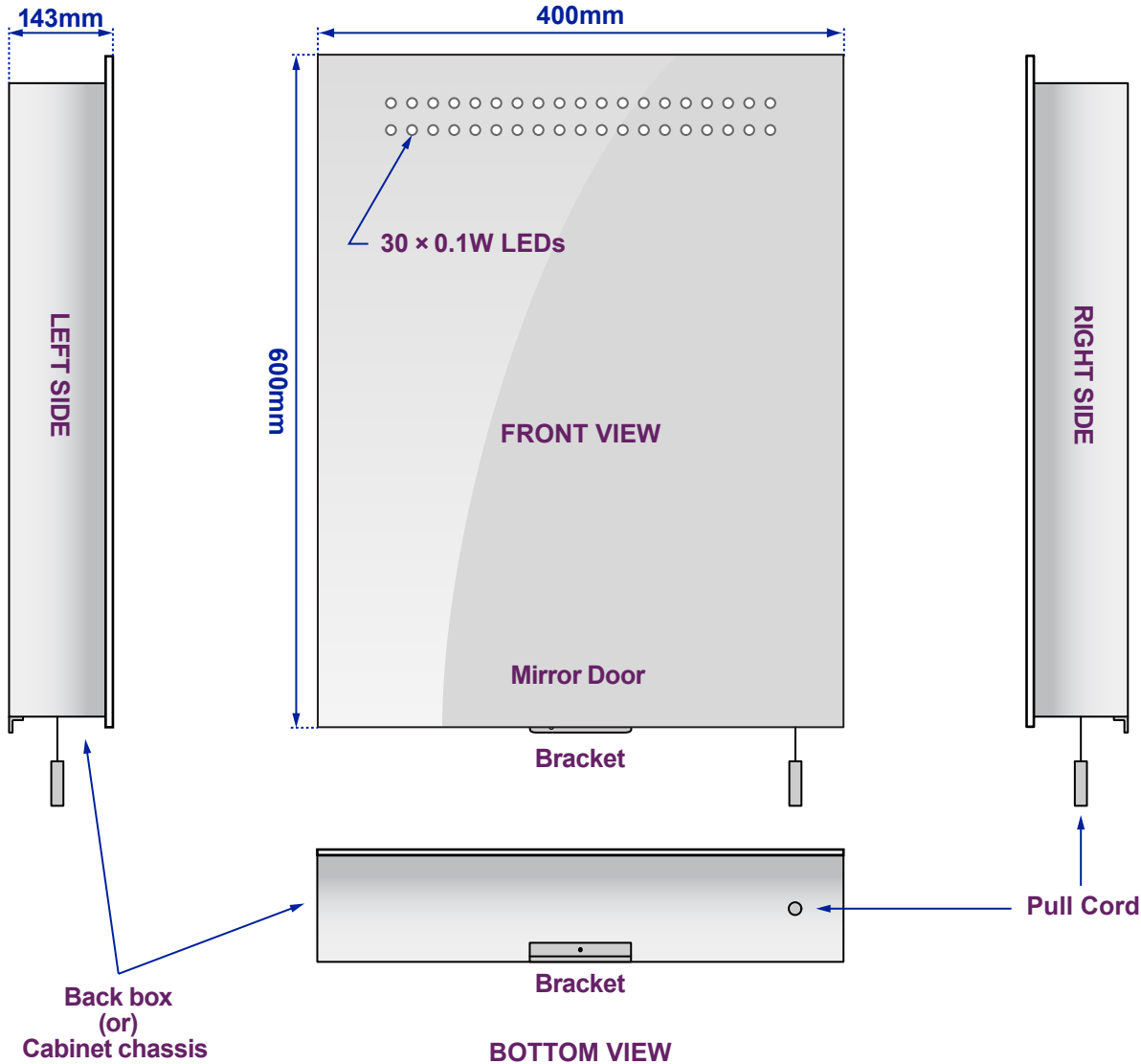
Views of complete assembly - With Mirror Door
