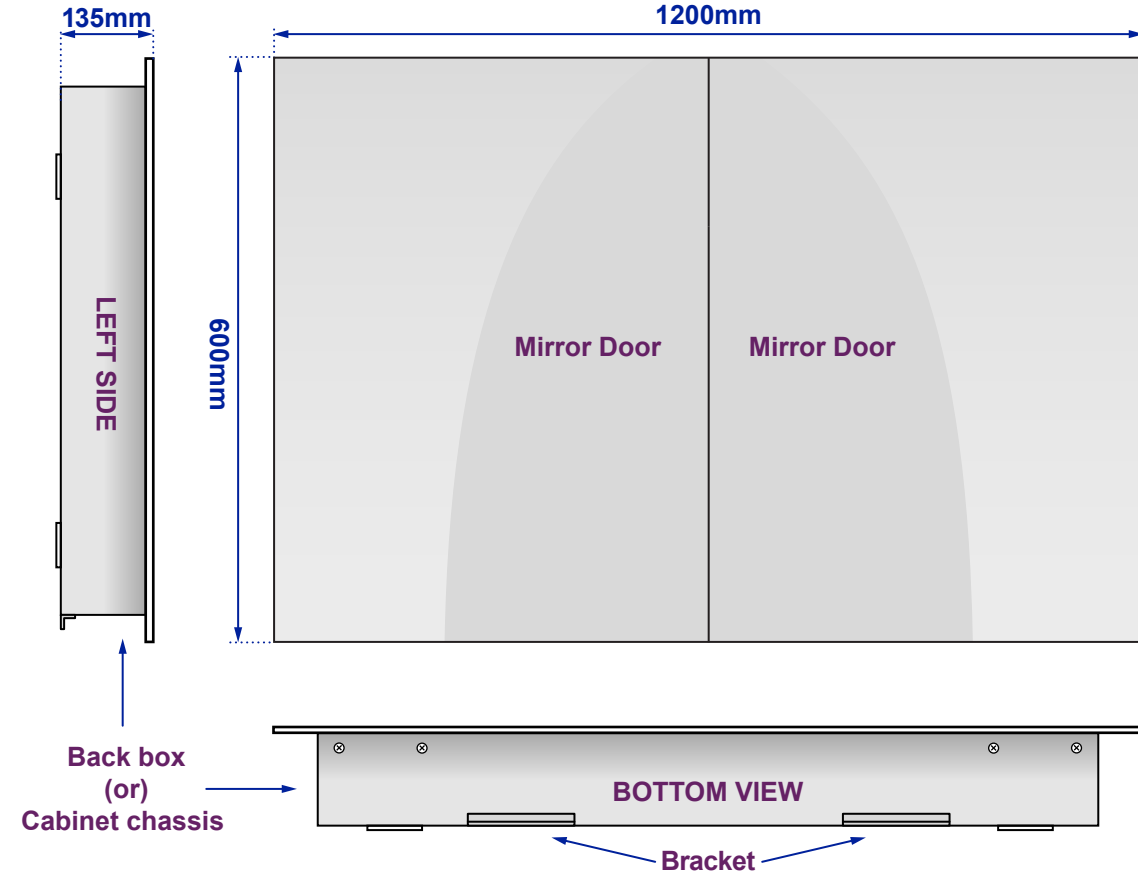
Views of complete assembly - With Mirror Door(s) / Panel(s)
