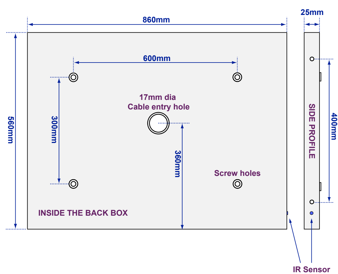
Views of Back plate - Without Mirror
