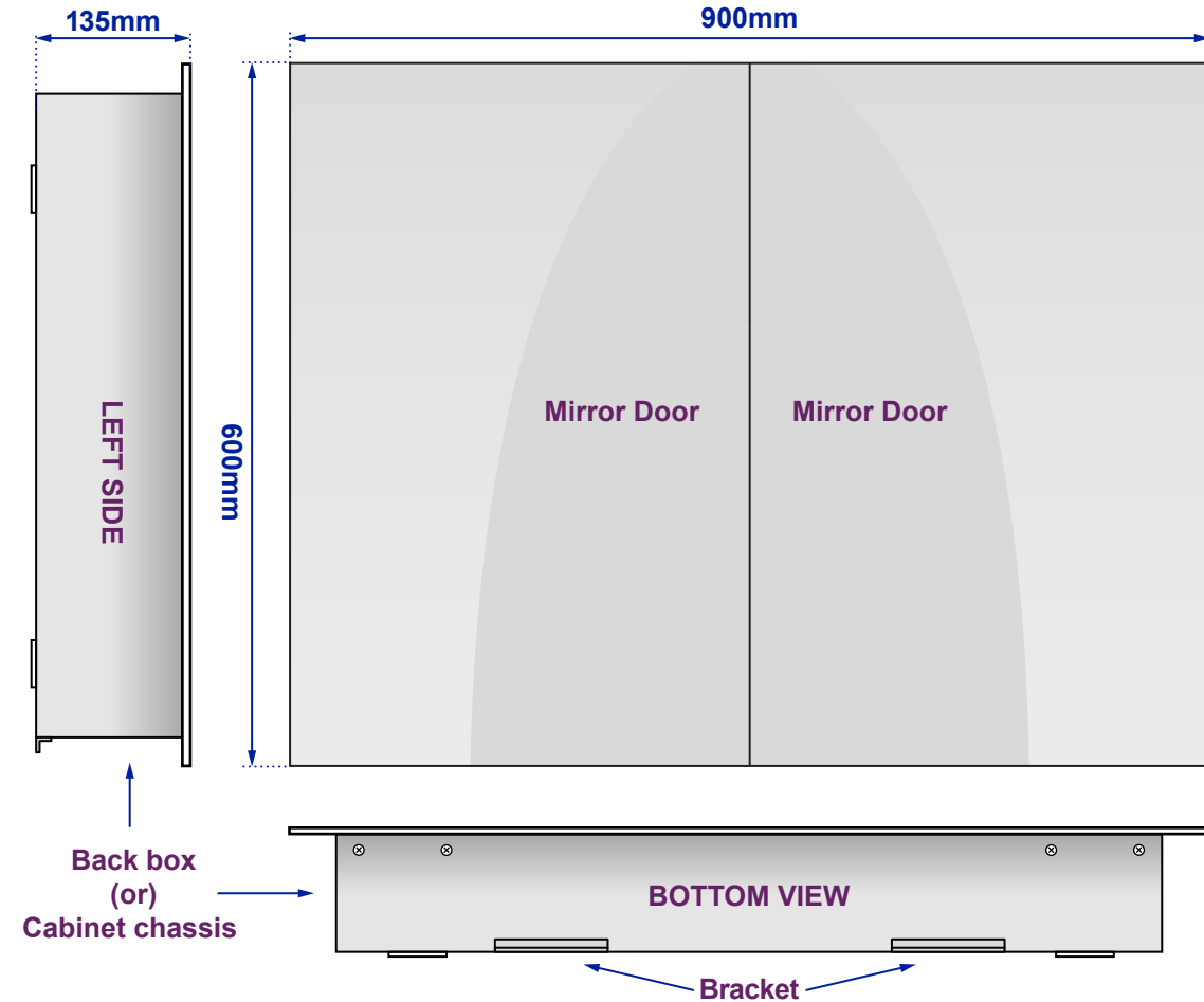
Views of complete assembly - With Mirror Door(s) / Panel(s)
