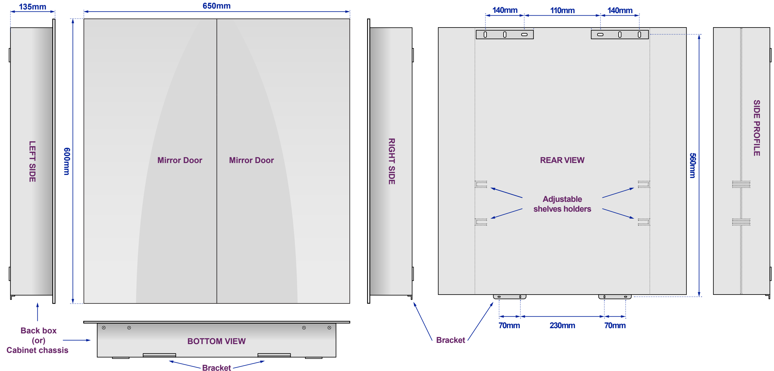
Views of complete assembly - With Mirror Door(s) / Panel(s)
